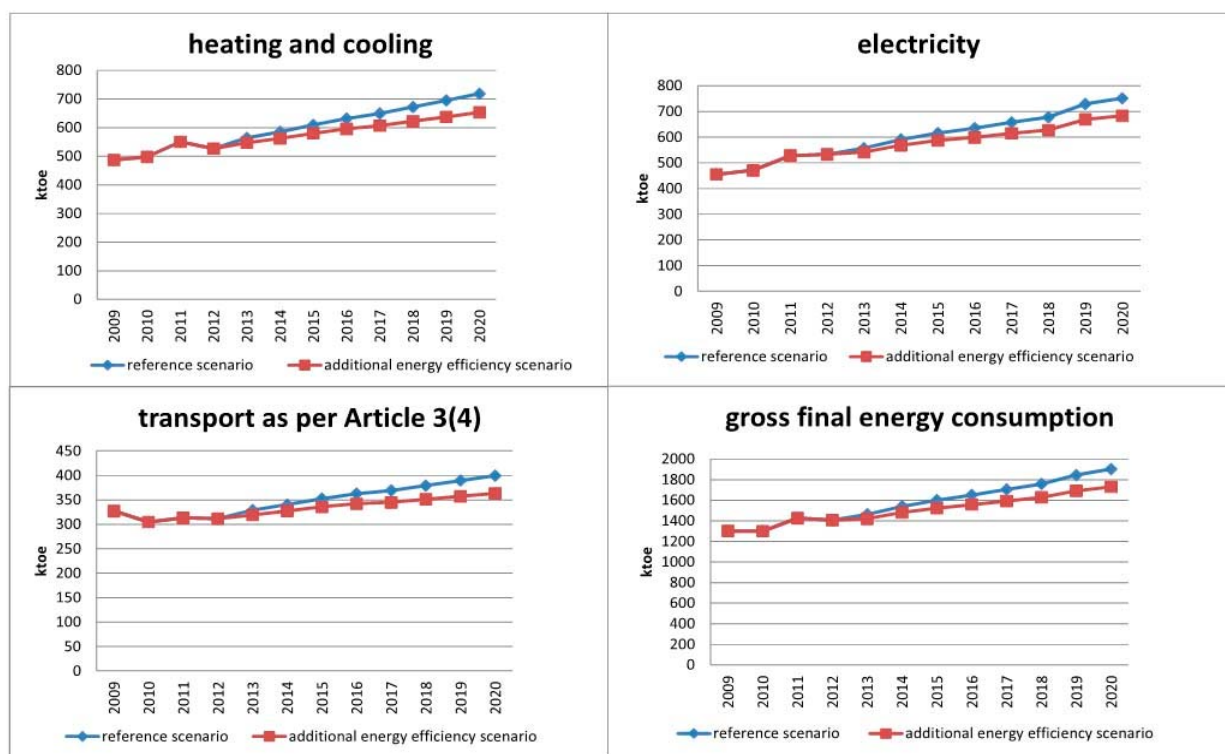
Figure 1 – Gross final energy consumption estimates in reference and additional energy efficiency scenarios until 2020
